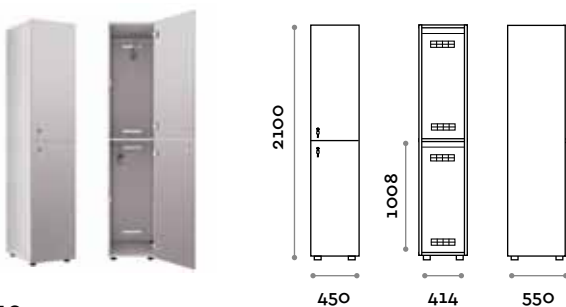
ANB03-19 Single column locker with 2 L-shaped doors
