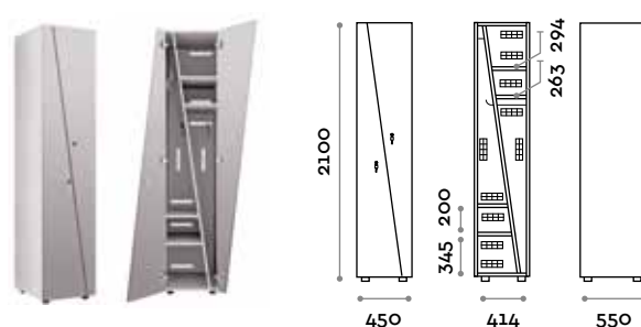
ATRO2-19 Single column locker with 2 trapezoidal doors
