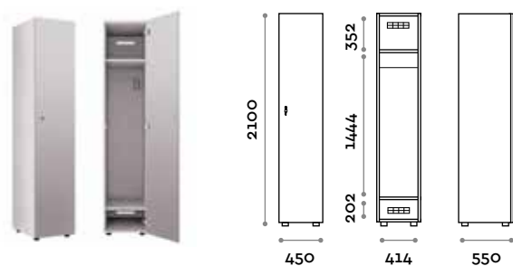
ANB02-19 Single column 2-tiers locker
