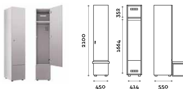
ANB12-19 Single column 2-tiers locker-bench version
