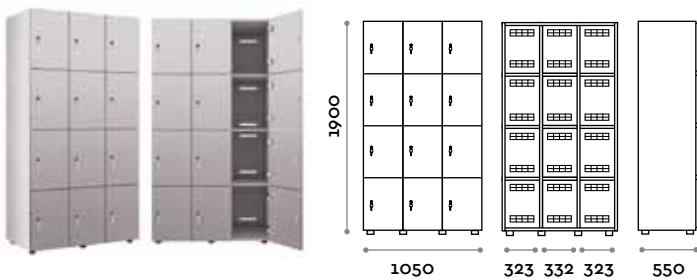
MAS4T Casier triple 12 portes
