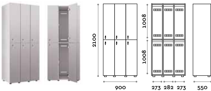
ANB90-19 Triple column 2-tiers locker, 6 doors
