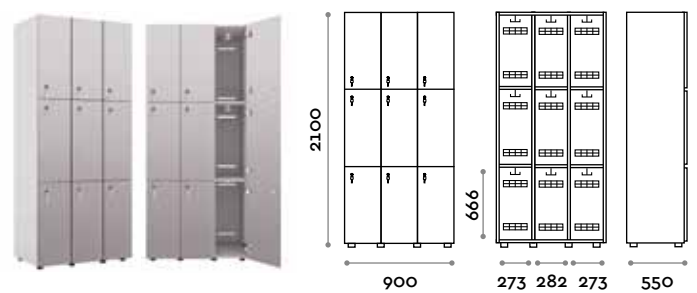
ANB93-19 Triple column 3-tiers locker, 9 doors with hook
