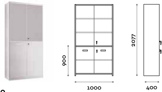
MB100 2-door cupboard with lock
