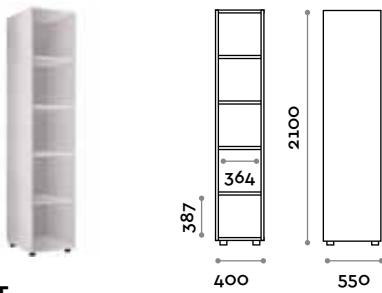
ACCDRT Clean/dirty towel unit with lockable door, two open racks and aluminium hole
