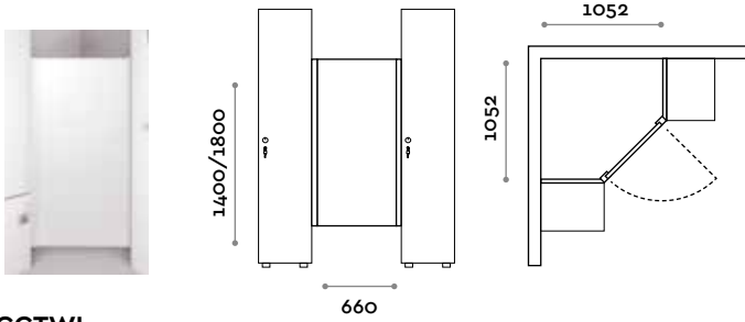
ACCTWL Towel storage unit with 4 racks
