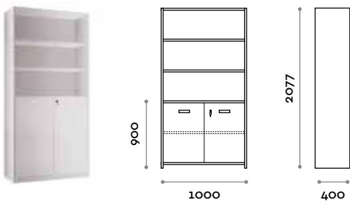
MA100 Cabinet with open shelves and doors
